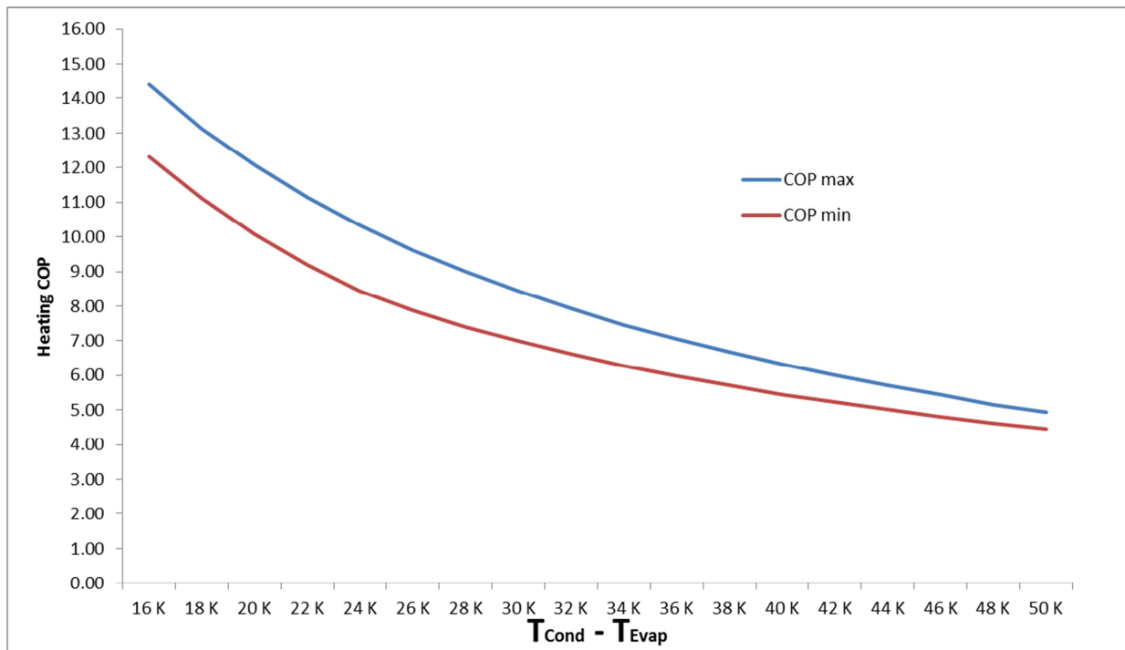
Figure 2: The heating coefficient of performance (COP) as function of the temperature difference between source and output temperature for high-efficiency ammonia heat pumps
